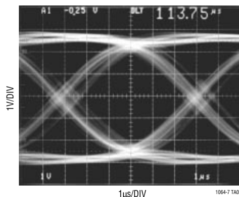
Eye Diagram
